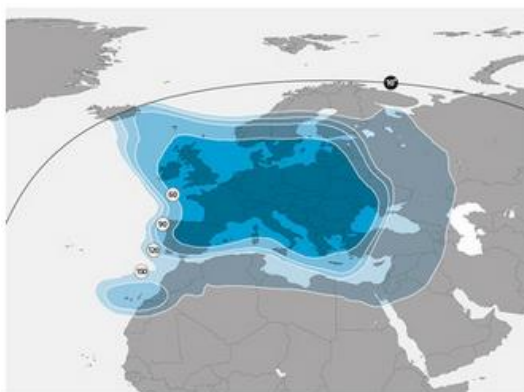
Europe Ku-band wide beam
